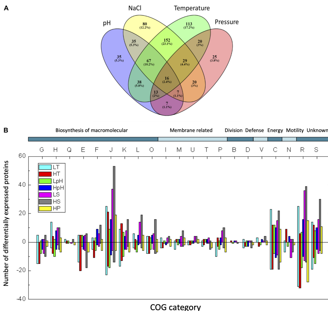
FIGURE 2 | (A) Venn diagram of DEP numbers under different stress conditions. Temperature, union of significant DEPs at both low and high temperature stress; NaCl, union of significant DEPs under LS and HS; pH, union of significant DEPs under LpH and HpH; Pressure, significant DEPs at HP stress. Percent of the total DEPs in all tested stresses is shown in parenthesis. (B) COG classification of DEPs. The following COG categories were included: G, carbohydrate transport and metabolism; H, coenzyme transport and metabolism; Q, secondary metabolite biosynthesis, transport, and catabolism; E, amino acid transport and metabolism; F, nucleotide transport and metabolism; J, translation, ribosomal structure, and biogenesis; K, transcription; L, replication, recombination, and repair; O, post-translational modification, protein turnover, and chaperones; I, lipid transport and metabolism; M, cell wall/membrane/envelope biogenesis; U, intracellular trafficking, secretion, and vesicular transport; T, signal transduction mechanisms; P, inorganic ion transport and metabolism; B, chromatin structure and dynamics; D, cell cycle control, cell division, and chromosome partitioning; V, defense mechanisms; C, energy production and conversion; N, cell motility; R, general function prediction only; S, function unknown. The numbers of up- or down-regulated proteins are indicated as bars with positive or negative numbers on the histogram, respectively.
