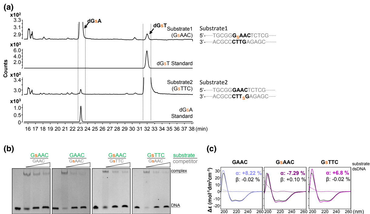
FIGURE 4 DNA PT modification at the GTTC side. (a) HPLC traces showing PT reaction with substrate DNA containing one PT modification. Substrate 1 contained a dGsA modification. Substrate 2 contained a dGsT modification. PT modification on the opposite side was then analyzed using HPLC/MS. For example, for substrate 1, dGsT was analyzed. (b) EMSA analysis of DndCDE binding to ds DNA with PT modification at one strand. Substrate DNA fluorescence is indicated by green color. Cold DNA is indicated with gray color. Ten- or 20-fold more unlabeled cold DNA was used for the experiments. (c) CD spectra of DndCDE protein binding to DNA with PT modification at one of the ds strands [Colour figure can be viewed at wileyonlinelibrary.com ]
