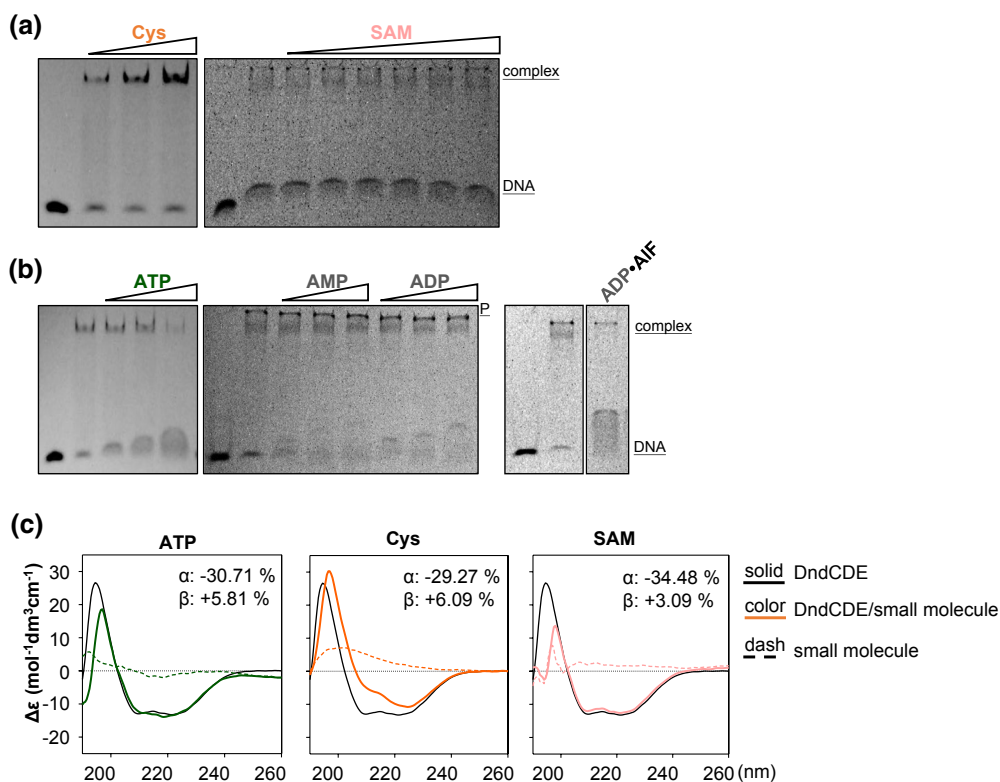
FIGURE 5 Effects of small molecules on DndCDE conformation and DNA complexation. In these experiments, 1 mM (if not indicated specifically) small molecules were used. In addition, 3.38 \mu M DndCDE and 0.4 \mu M DNA were used in the EMSA study. (a) EMSA analysis of DndCDE binding to substrate DNA in the presence of ATP, ADP, AMP, (2.5, 5.0 and 7.5 mM, respectively) and ADP•AIF (7.5 mM). (b) EMSA analysis of DndCDE binding to substrate DNA in the presence of cysteine (0, 1 and 2 mM) and SAM (0–6 mM). (c) CD spectra of DndCDE in the presence of ATP, Cys and SAM. DndCDE (0.2 \mu M) in CD buffer was used for the study [Colour figure can be viewed at wileyonlinelibrary.com]
