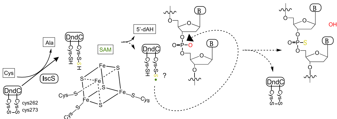
FIGURE 6 Pathway for the formation of PT. Small molecules are indicated by squares. Proteins are indicated by round corner squares. The perthiyl radical is indicated by the green dot. The dashed arrows indicate the suggested chemical steps that need to be investigated [Colour figure can be viewed at wileyonlinelibrary.com]
