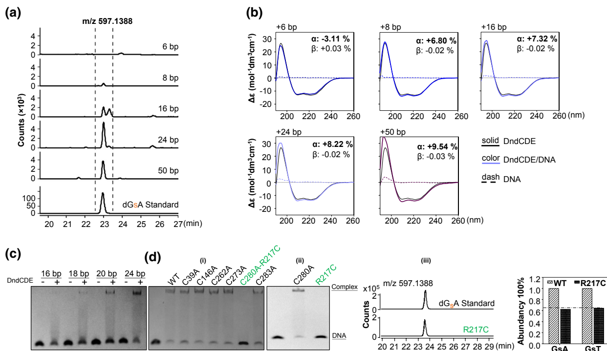
FIGURE 3 DNA chain length requirement for PT reaction. (a) HPLC traces showing DNA substrates with increasing chain length and the yield of dGsA from PT. (b) Circular dichroism spectra of DndCDE protein upon binding to DNA substrate. The content of \alpha -helices and \beta -strands were analyzed using K2D3 software. (c) EMSA analysis of DndCDE binding to DNA of increasing chain length. (d) Mutational analysis of DNA binding by DndCDE and the related PT activity. (i) DNA binding by DndCDE with mutation of cysteine residues on DndC. The green color marks the accidental introduction of an arginine residue mutation in DndD. (ii) DNA binding by DndCDE with the site-directed mutation on DndC or DndD. (iii) HPLC traces showing DNA PT modification by DndD R217 mutant. The columns show the percentage of PT modification in DndD R217 mutant relative to the wild type [Colour figure can be viewed at wileyonlinelibrary.com ]
